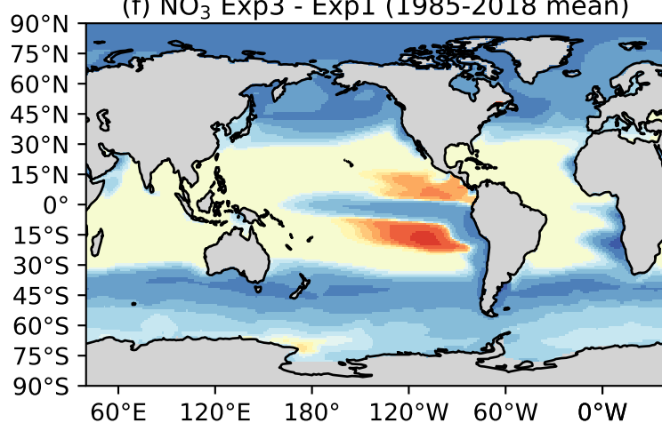
(f) NO 3 Exp3 - Exp1 (1985-2018 mean)
