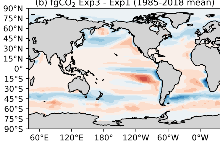
(b) fgCO 2 Exp3 - Exp1 (1985-2018 mean)
