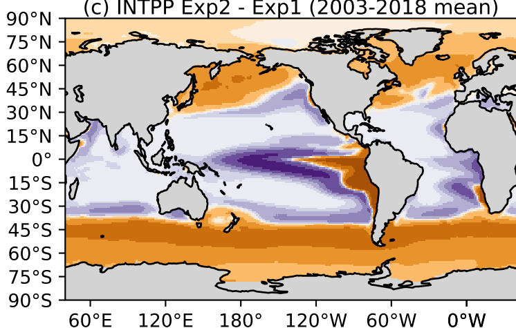
(c) INTPP Exp2 - Exp1 (2003-2018 mean)
