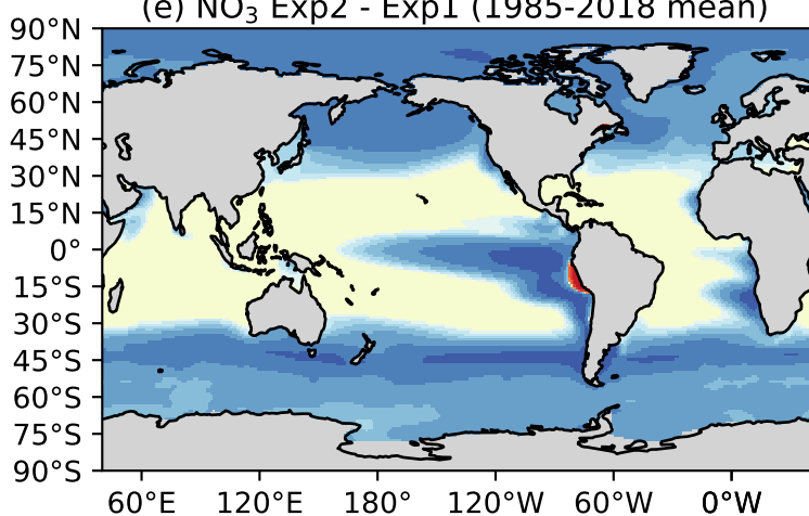
(e) NO 3 Exp2 - Exp1 (1985-2018 mean)
