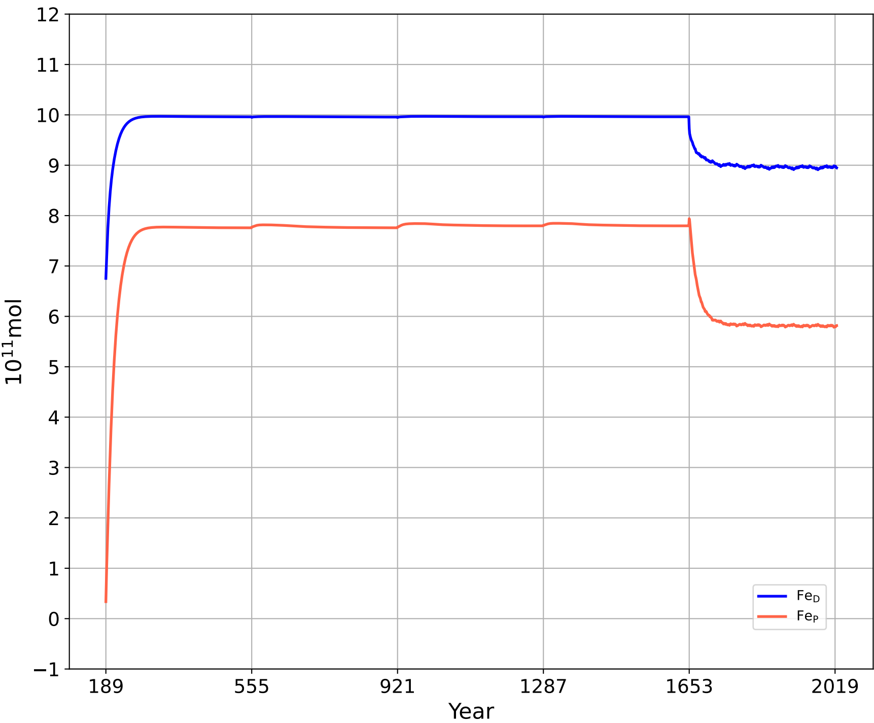
Fe D and Fe P integrated over the global ocean
