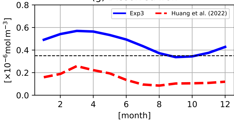
(g) Dissolved Iron
