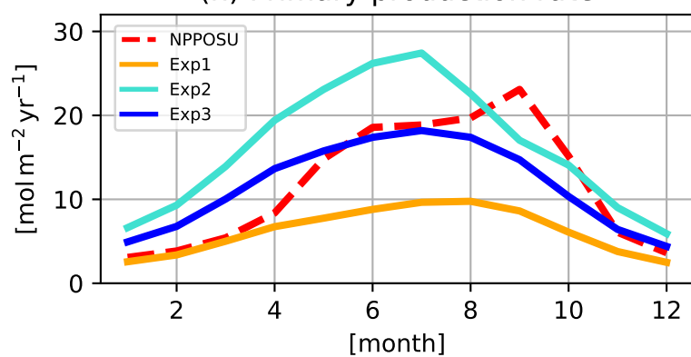
(h) Primary production rate
