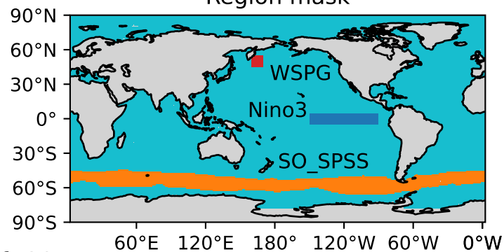
(a) \text{fgCO}_2
