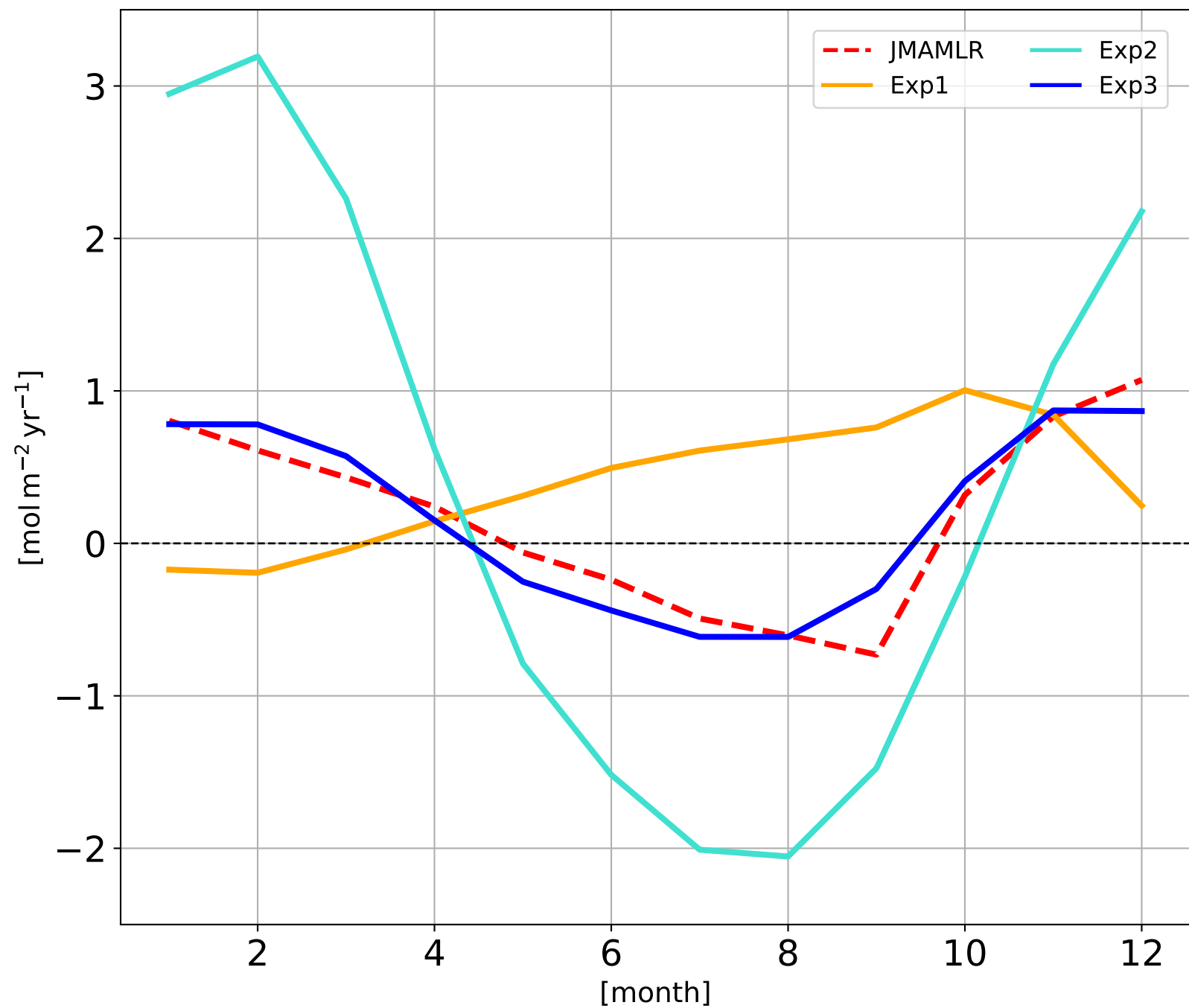
FgCO 2 (positive into the ocean) SO_SPSS
