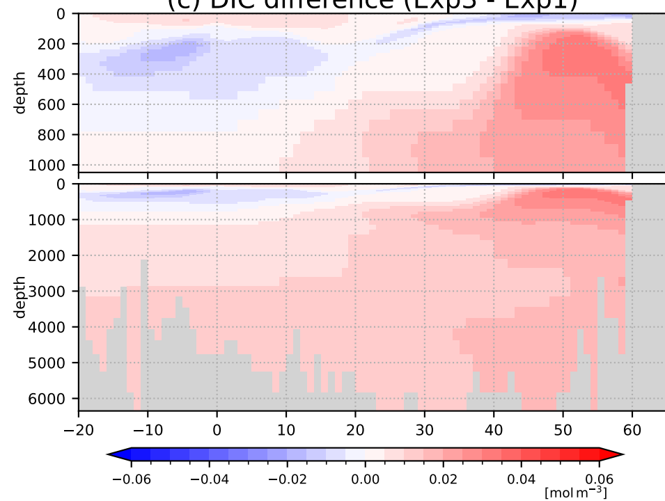
(c) DIC difference (Exp3 - Exp1)
